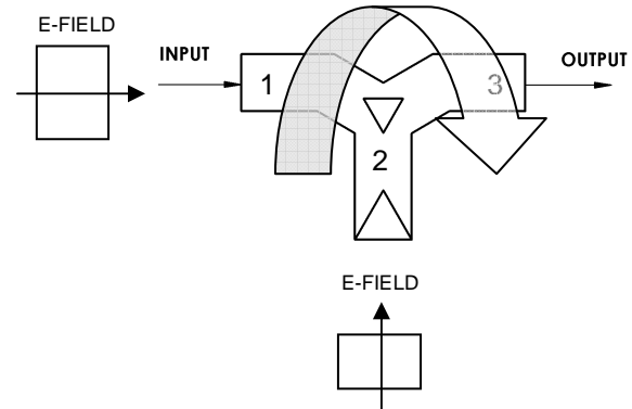
Port Orientation Option S
